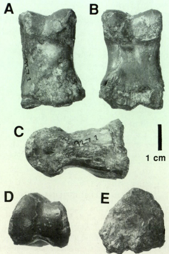
Figure 1 Theropod pedal phalanx, proximal element of fourth digit, left side. WAM 92.7.1.Molecap Greensand (Late Cretaceous), Molecap Quarry, Gingin, Western Australia. Specimens shown in A, dorsal; B, ventral; C, left lateral; D, distal and E, proximal views.
