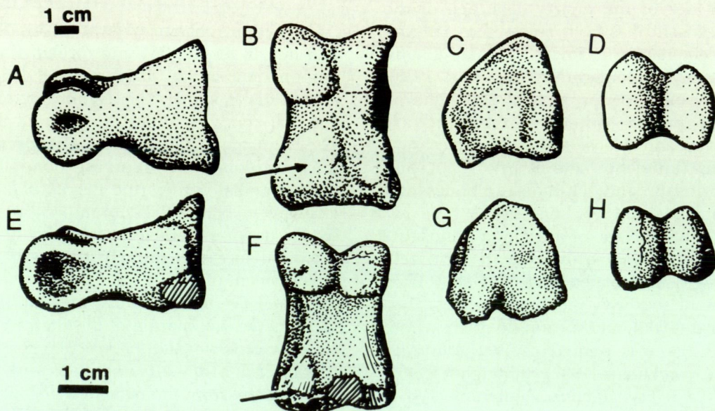
Figure 2 Comparison between the left fourth pedal proximal phalanx in Allosaurus fragilis (A-D) and the Gingin theropod (E-H). A, E, lateral views; B, F, ventral views, arrow points to flexor tubercle; C, G, proximal face; D, H, distal view of articular condyles. A-D after Madsen (1976).
